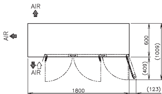
VIEW A(1/10)
